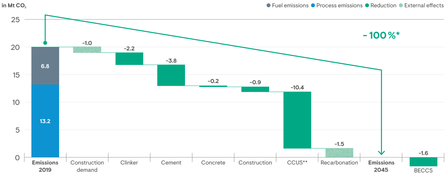
Fig. 3: Scenario climate neutrality – CO 2 reduction by 2045
