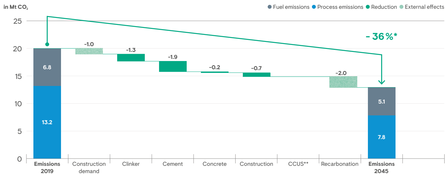
Fig. 2: Ambitious reference scenario – CO 2 reduction by 2045
